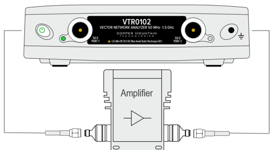
Amplifier Evaluation
