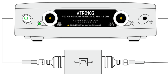
Filter Characterization
