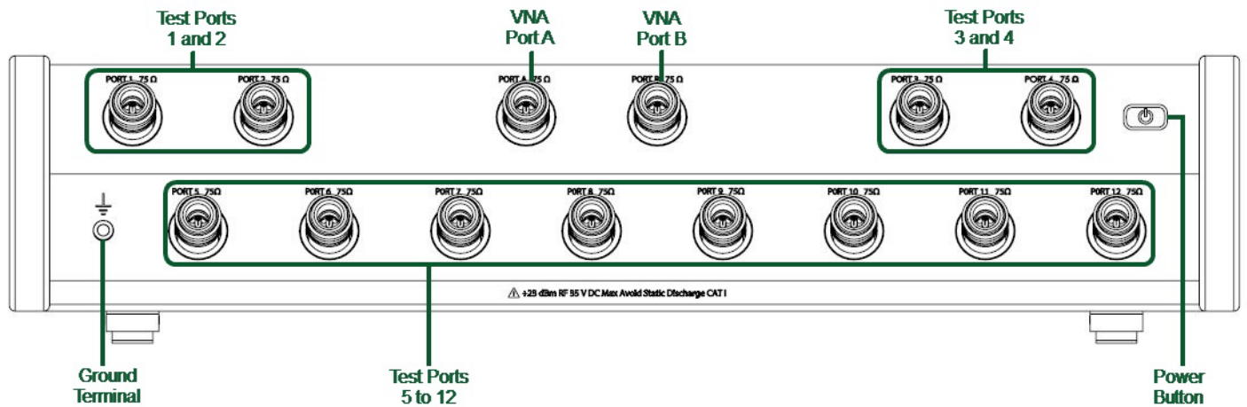
Front Panel
